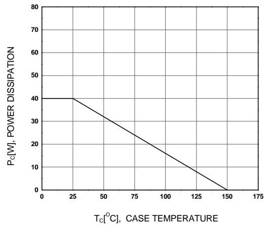
Figure 6. Power Derating
